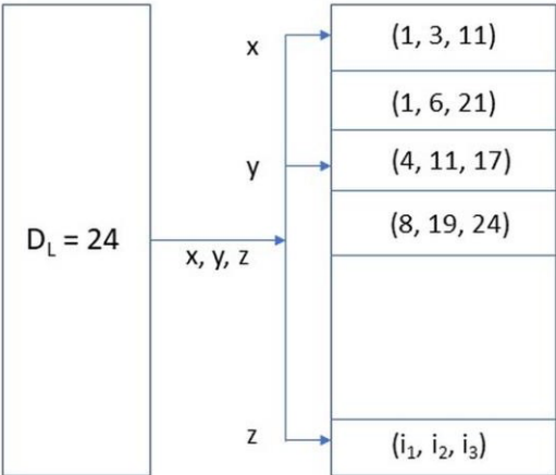
Figure 3: Stacked structure of latent activations
