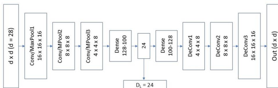
Figure 1: Convolutional autoencoder with dimensionality reduction.
