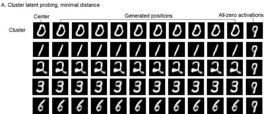
Figure 5: Latent probing of landscape features. Distances: d1 = 0.05; d2 = 0.1; d3 = 0.15 Dg
