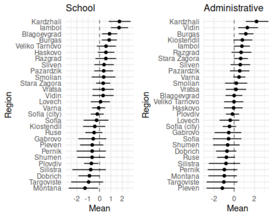
Figure 1: Posterior means and 95% credible intervals of region-level intercepts for school- and administrative e-services. University and private services are omitted for brevity.
